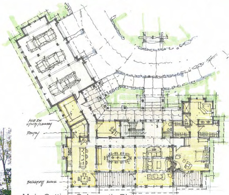
Main Cottage Schematic Plan
